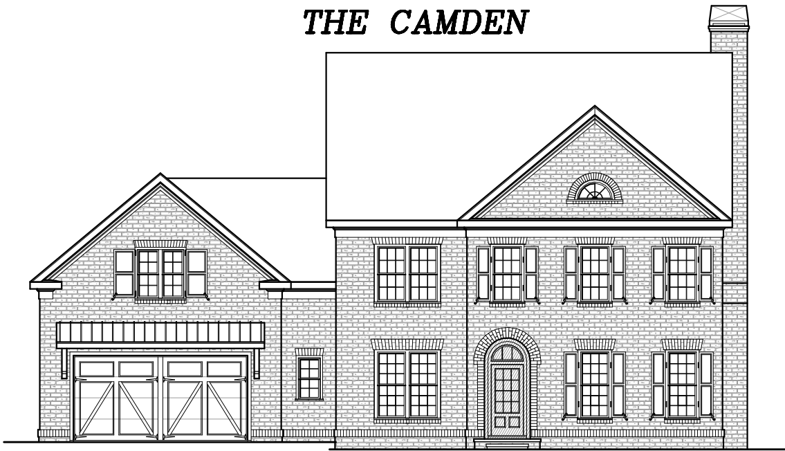
STREET ELEVATION
