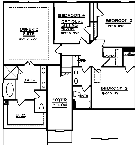
SECOND FLOOR
