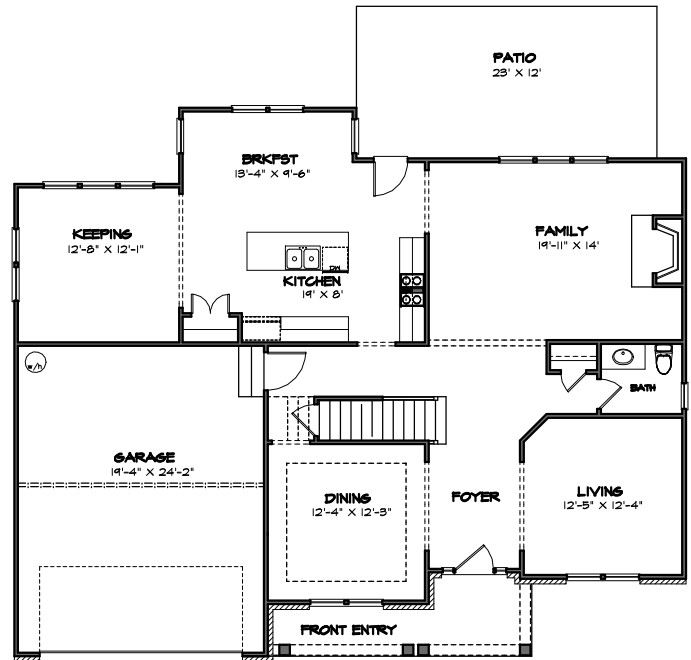
MAIN LEVEL
